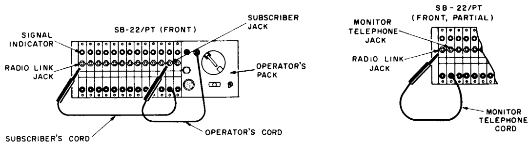
C. CORD CONNECTION FOR MONITOR TELEPHONE (NOTE 2).
