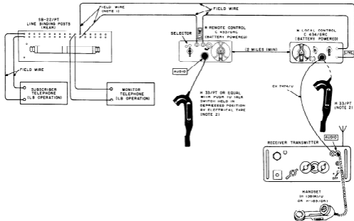
Figure 6-18. AN/GR-6 and receiver-transmitter remote radio control and RWI connections and control settings
