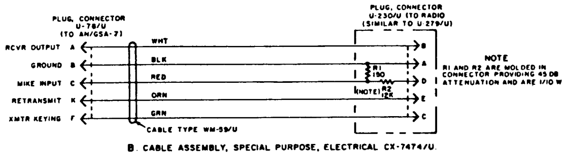
B. CABLE ASSEMBLY, SPECIAL PURPOSE, ELECTRICAL CX-7474/U.
