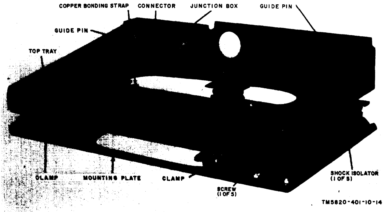
Figure 1-8. Mounting MT-1029/VRC.
