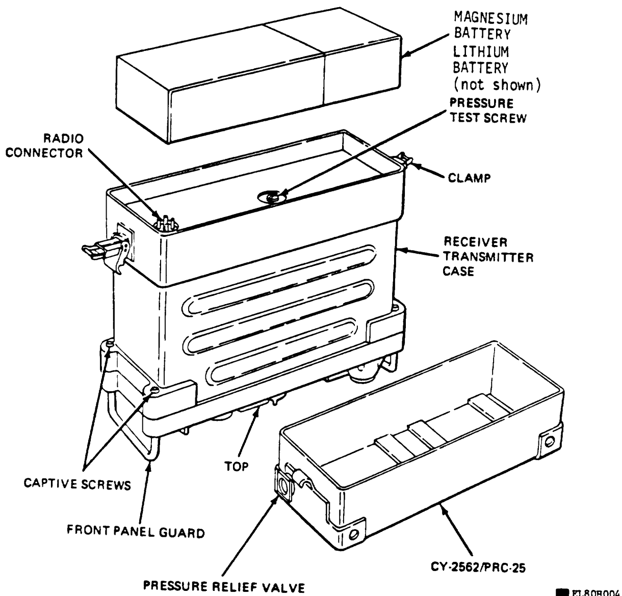
■ Figure 2-6. Installing battery in receiver-transmitter.
